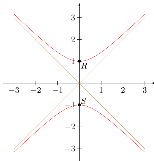
FIGURE 12.7: La courbe de niveau x^2 - y^2 = -1 .
